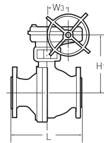
Size DN 150 to 200 Full bore
