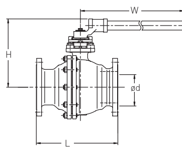
Size DN 125 to 200 Full bore
