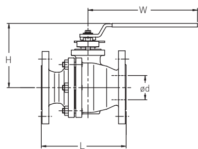
Size DN 15 to 100 Full bore
